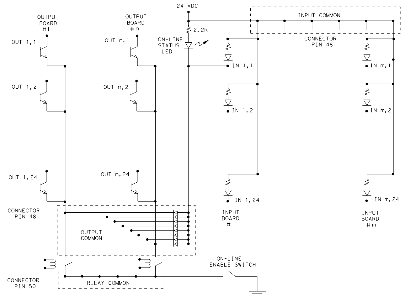
INTERIOR FRONT PANEL SCHEMATIC
