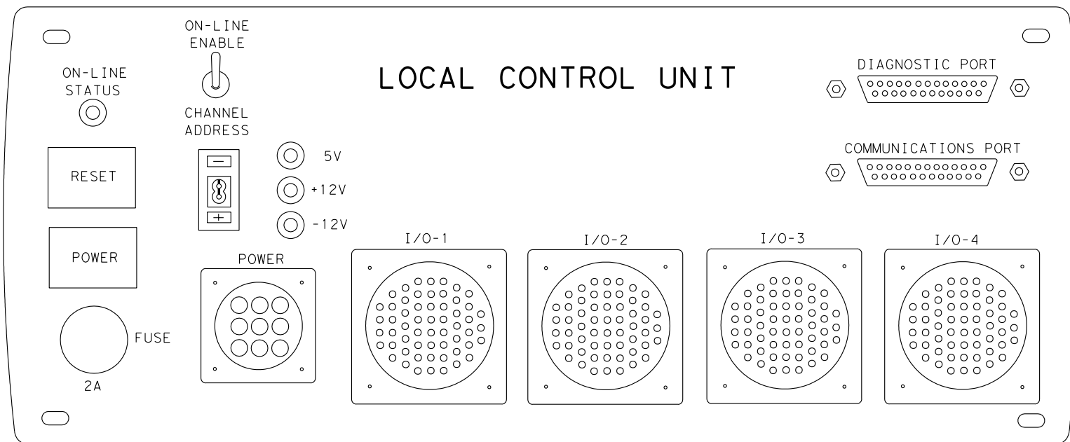
LCU FRONT PANEL
